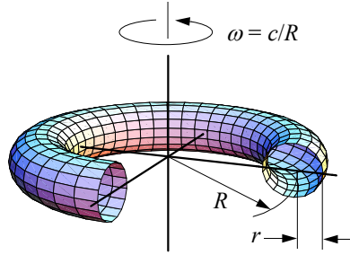
Figure 1: The Spinning Ring Model of the Electron
